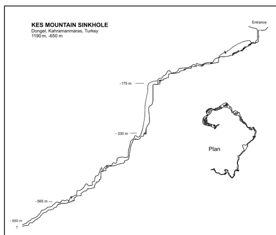
Fig 2: Kes Mountain Sinkhole, 2011
