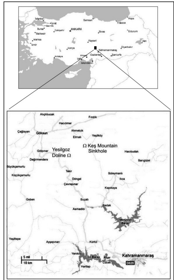
Fig. 1: Kes Mountain Sinkhole, Yesilgoz Doline and the area in general
