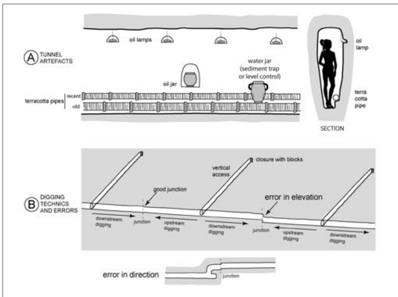
Fig.7: A) tunnel artefacts like oil lamp niches and terracotta pipes. B) digging technics and some errors at the junctions (drawing E. Gilli).
